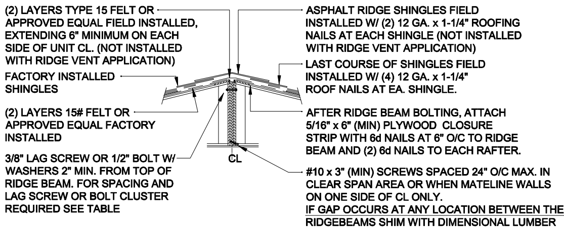
RIDGE CLOSE - UP DETAIL - SHINGLE ROOF
