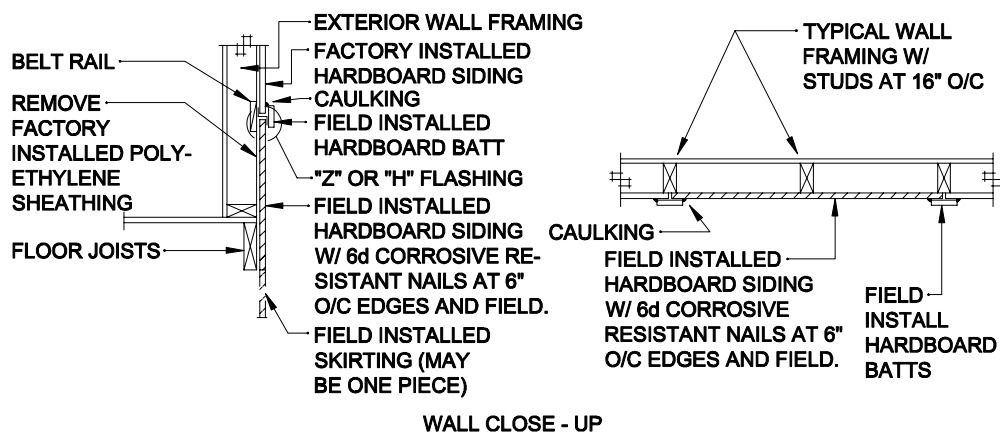
Figure 19C. Wall close-up
