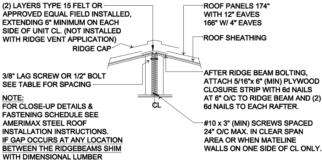
RIDGE CLOSE - UP DETAIL - METAL ROOF
