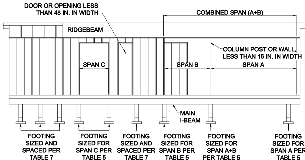
Figure 1. Typical point-load support locations along the marriage line.
