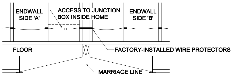
Figure 43. Inside partition or end wall electrical crossover connection
